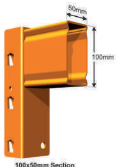
100x50mm Section
