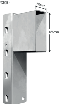
125x50mm Section
